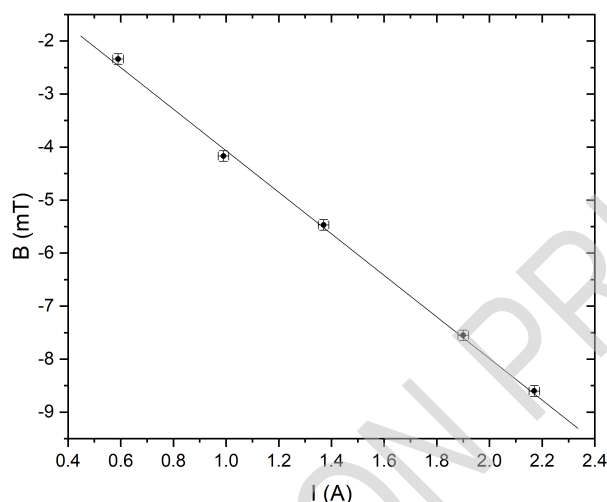
Magnetic slope at z=+28\text{mm} .
